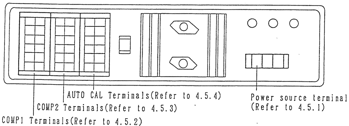
Fig.4.5.2 Rear panel
