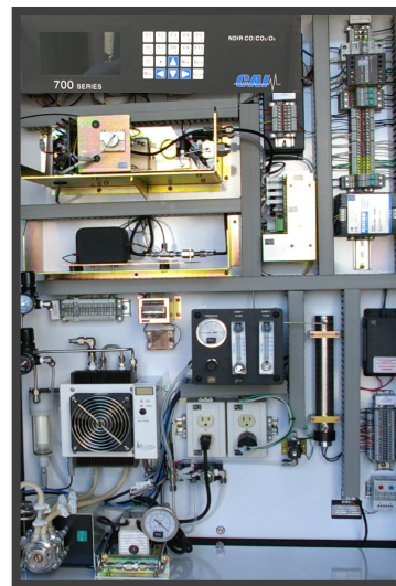
Internal View
